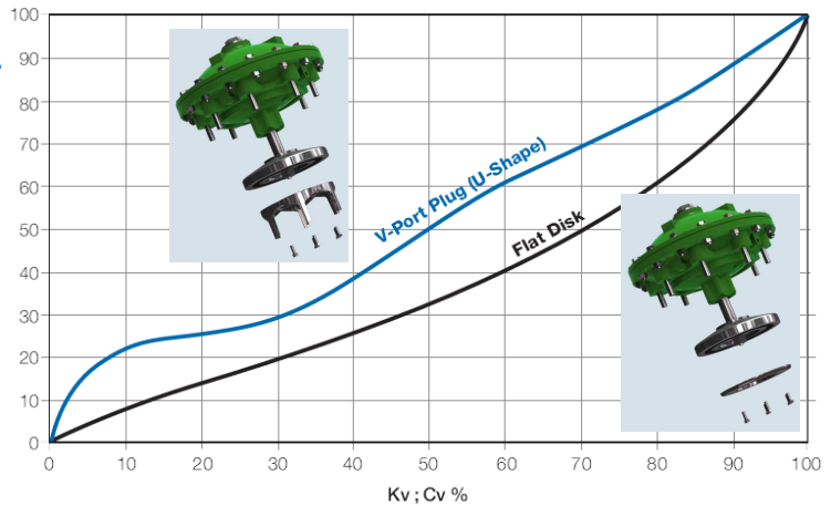
Kv ; Cv to Valve Opening Chart
